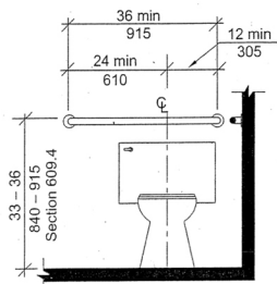
Rear Wall Grab Bar for Water Closet
