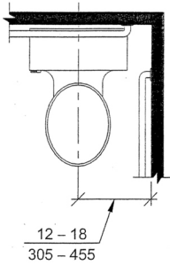
Children's Water Closet Location
