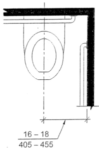
(a) Accessible Water Closets
