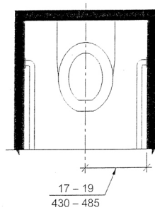
(b) Ambulatory Accessible Water Closets
