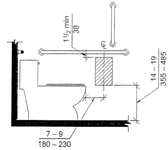
Children's Dispenser Location
