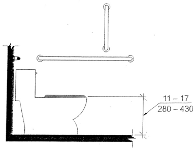
Children's Water Closet Height
