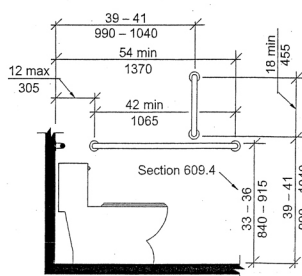
Side Wall Grab Bar for Water Closet
