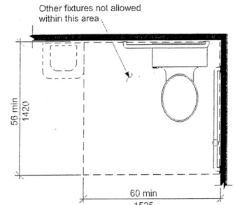
Size of Clearance for Water Closet
