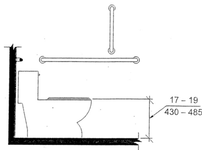
Water Closet Height
