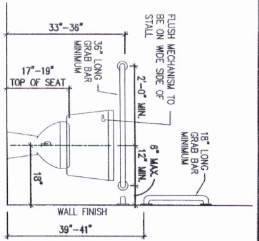
HC WATER CLOSET
